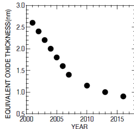
Fig. 1 Reduction of equivalent oxide thickness vs. year referred from the 2002 ITRS road map. This is an example.
